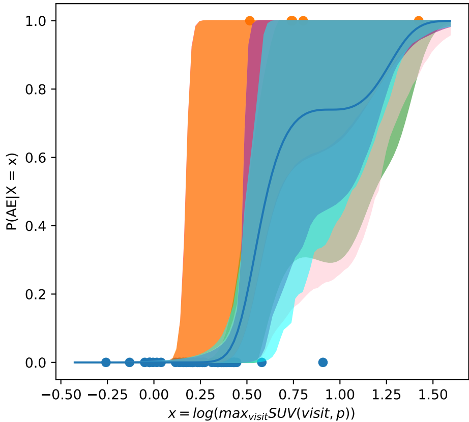
cond. prob. for AE: scale log
